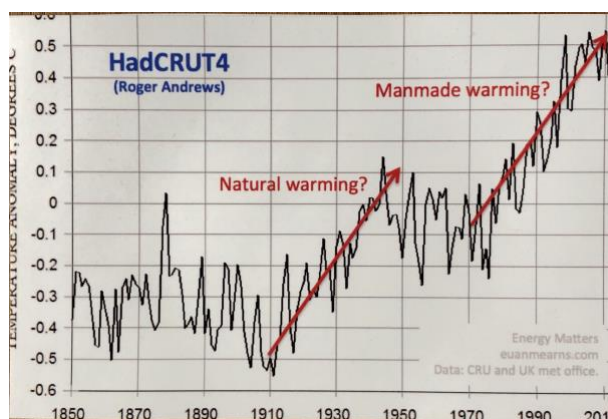
Figur 2: Temperaturanomalierna i grader
